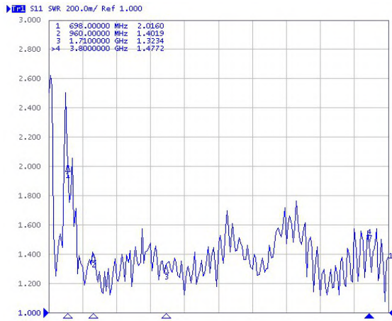
SWR Antenna 1
