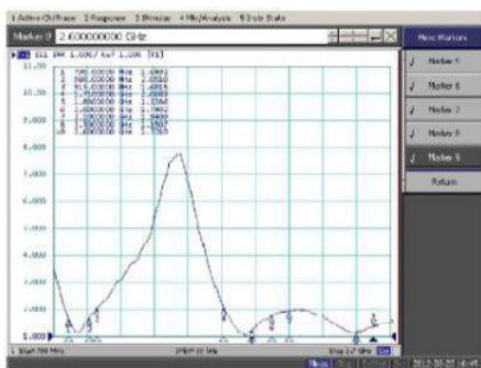
V.S.W.R CURVE MADE WITH MASS PLANE mm.260x90
