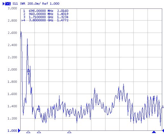
SWR Antenna 1
