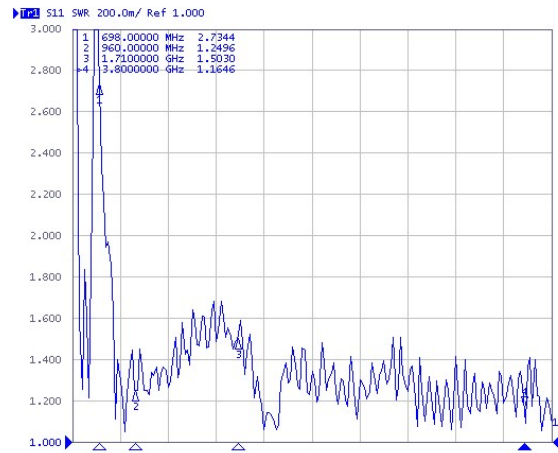
SWR Antenna 2
